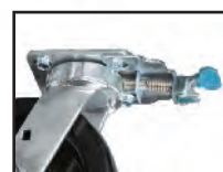
4 Position Swivel Lock
