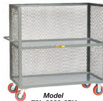
Model T3-3060-6PY 3 Shelf with Mesh Sides
